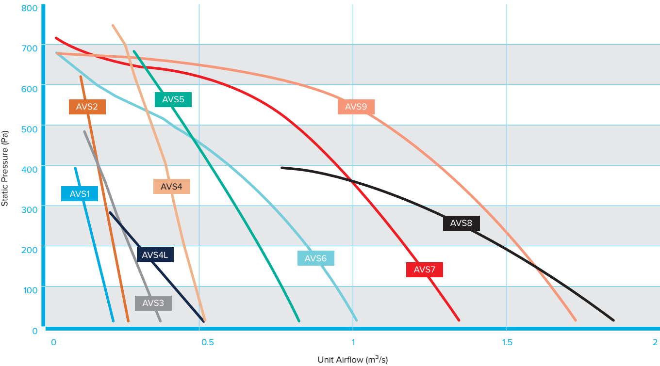
PERFORMANCE CHART
