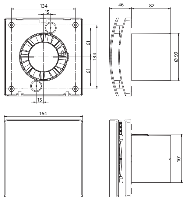
Figure 1. iSense Dimensions
