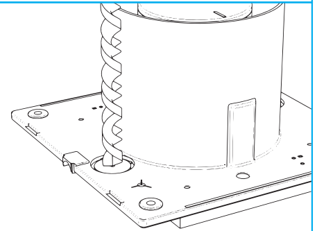
Figure 4. Drilling fan backplate for recessed cable entry.
