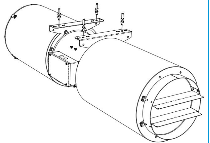
Figure 2. Mounting Points
