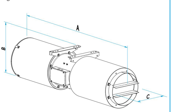
Figure 3. Unit Dimensions
