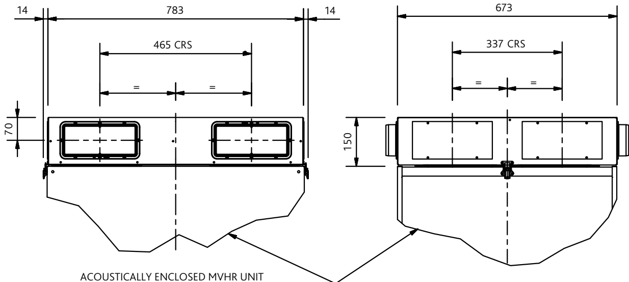
Figure 2. Dimensions.
