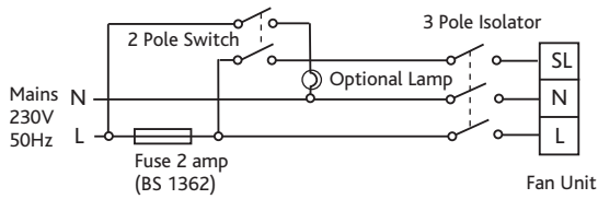
Figure 4d. Wiring. PCB details (where applicable)
