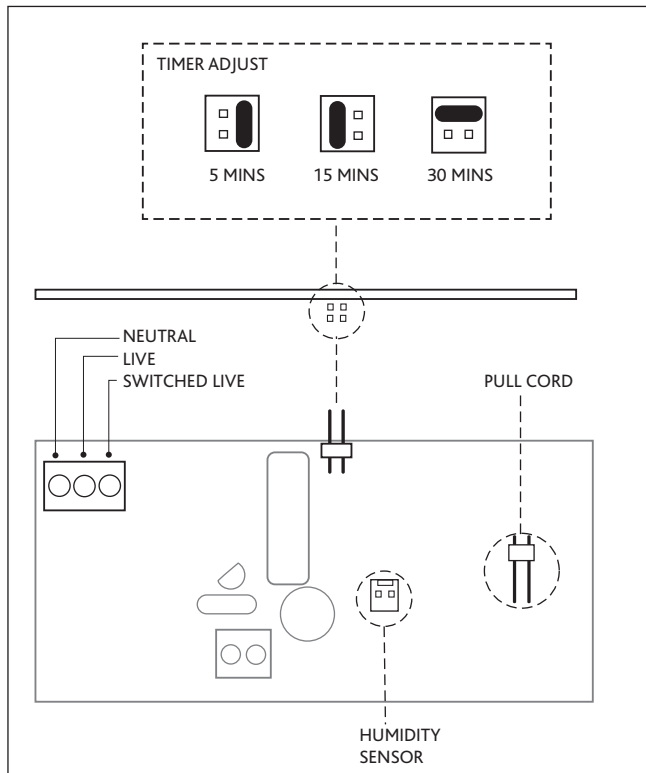
Figure 4d. Wiring. PCB details (where applicable)
