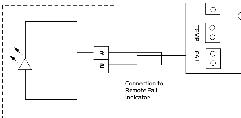
Figure 2. Fan terminal block
