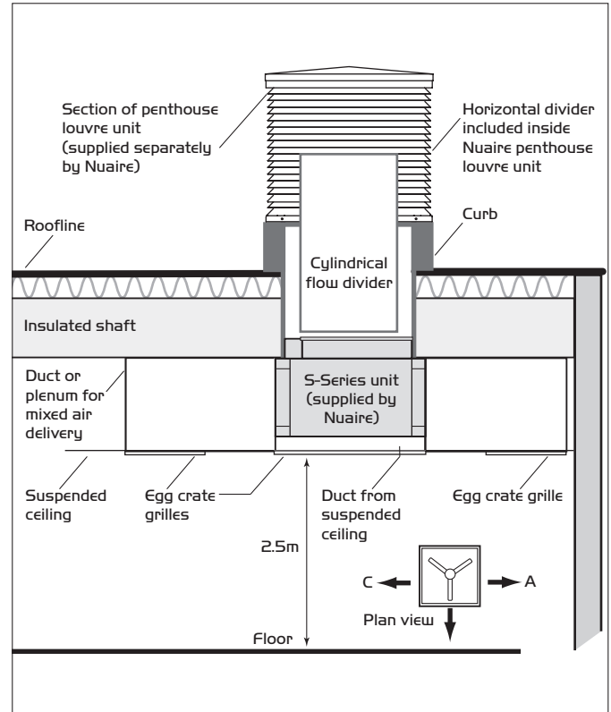
Figure 6b. (Section view of unit installed above a suspended ceiling in conjunction with a roof terminal and shaft with insulation removed for clarity).
