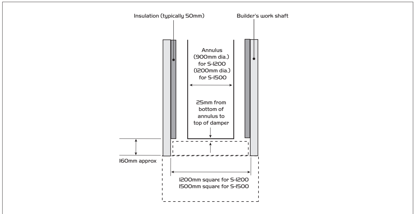
Figure 7. Typical square shaft detail.
