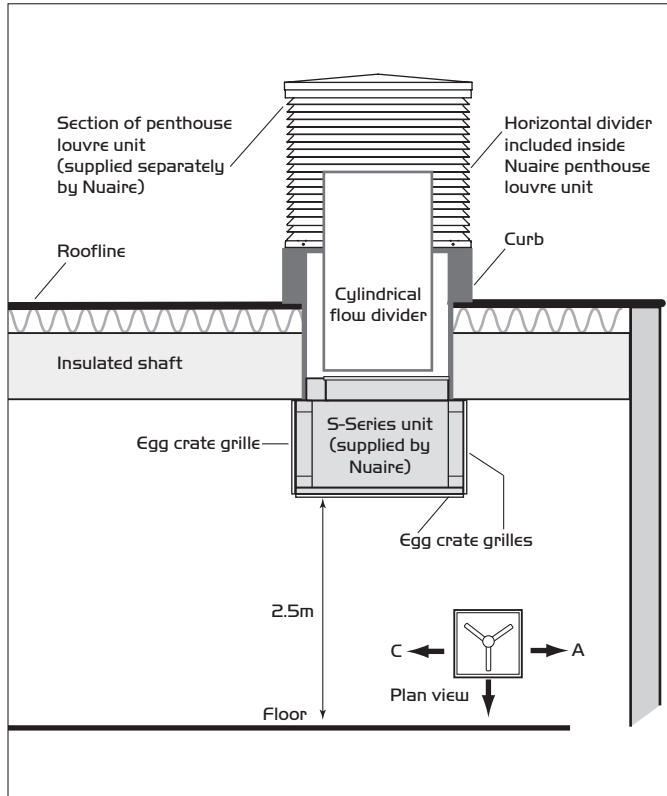
Figure 7. Typical square shaft detail.
