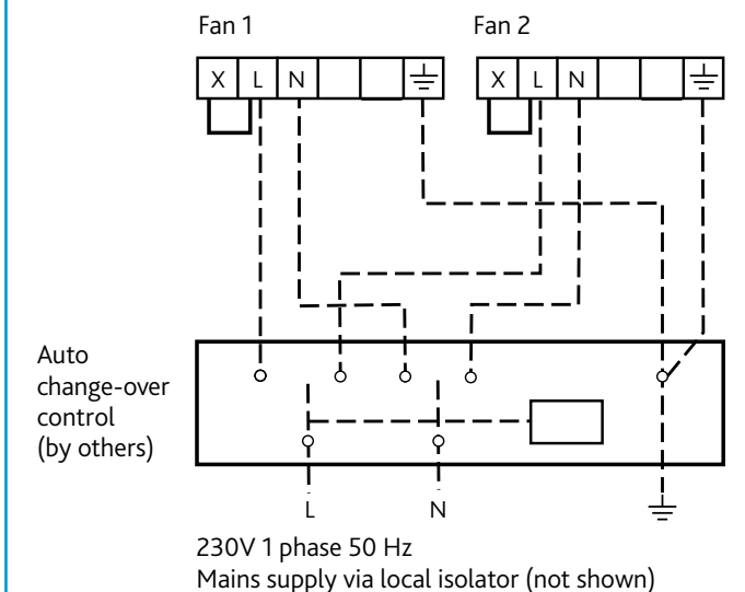
Figure 5. Single Phase Fans - Constant Speed.
