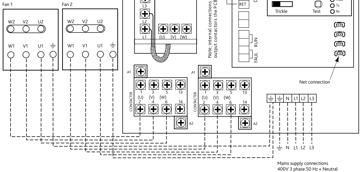
Figure 8. Single Phase Fans - with Ecosmart (ES-ISCT) controls, motors up to 3kW inclusive.
