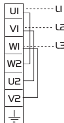
3 phase for DOL STARTING (4kW and above) 400V 3 phase 50Hz supply
