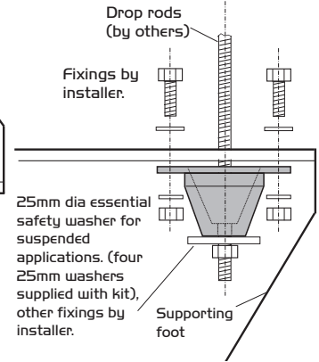
Figure 4. Resilient Mounting 'Suspended' fixing.
