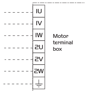
2 SPEED TAP/ PAM WOUND MOTOR (D.O.L. starting both speeds) Note: individual wiring instructions are included with each unit
