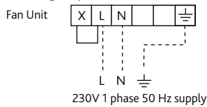
Figure 4. Single phase, single speed.
