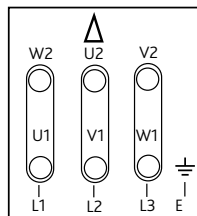
Figure 6. 3 phase units 4kW and above.
