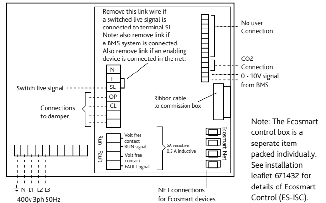
Figure 11. Set up/Commissioning Box
