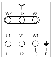
Figure 5. 3 phase units up to 3 kW.
