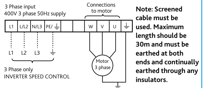
Figure 10. 3 phase (Ecosmart Control)
